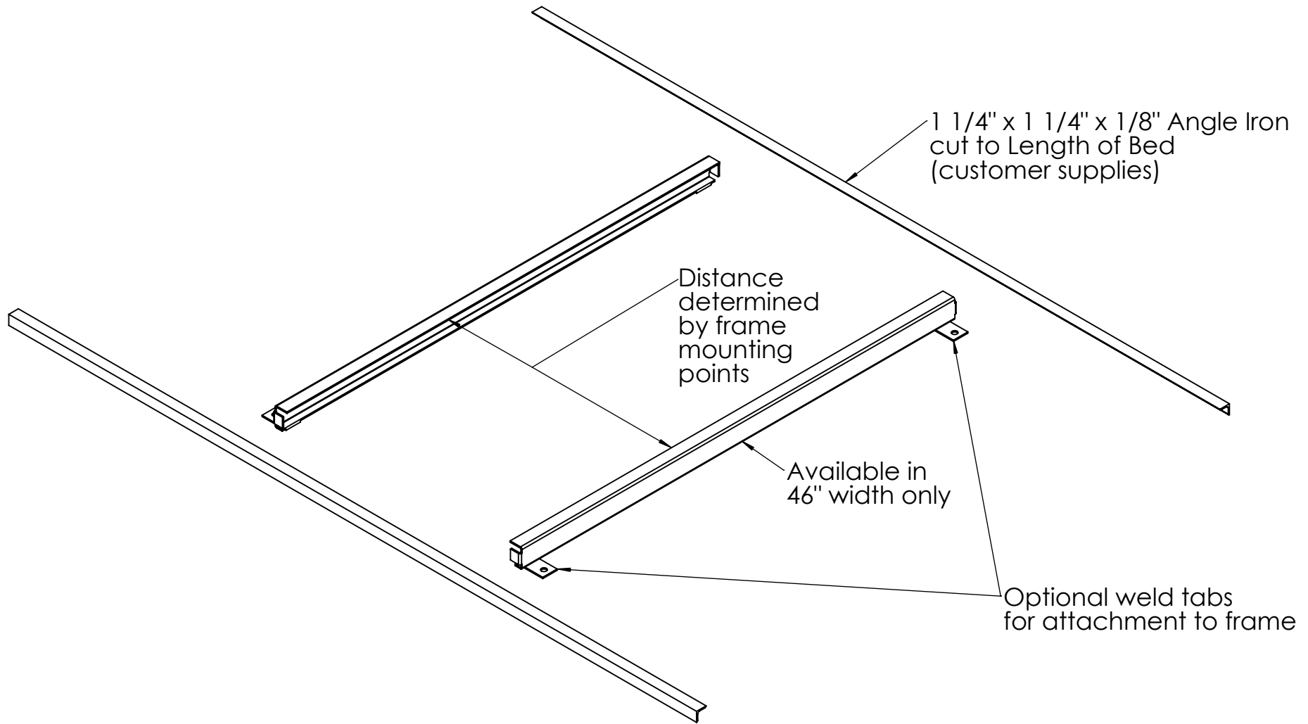
TYPICAL SUBFRAME ASSEMBLY
